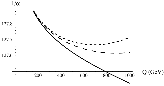
Fig. 1. The effective coupling as a function of Q , for \delta = 1 (solid), \delta = 2 (long-dashed), and \delta = 3 (short-dashed)
